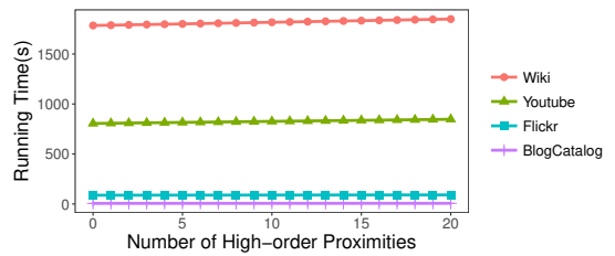
Figure 6: The running time vs. the number of high-order proximities. The results show that the running time increases very slightly with respect to the number of proximities.
