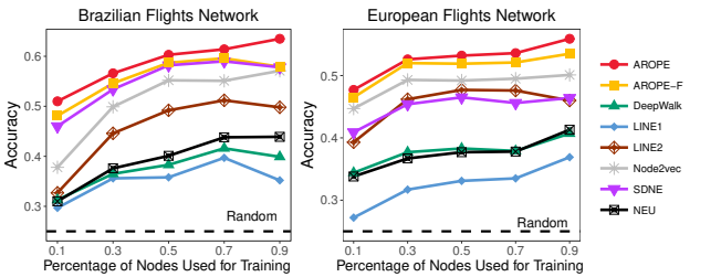
Figure 4: Results of node structural role classification on two flights networks. The results show that our method has higher accuracies, demonstrating better performance in capturing the structural role of nodes on these two networks.
