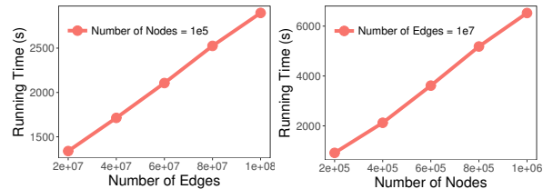
Figure 7: The scalability analysis of AROPE on synthetic networks. The results show that our method has a linear time complexity with respect to the number of nodes and number of edges respectively. In addition, our method is extremely efficient, which can be applied to real large-scale networks.
