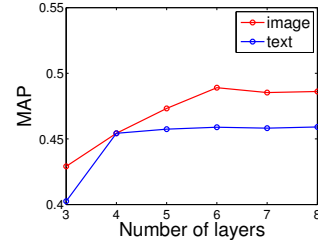
Figure 3: MAP for WIKI when setting the number of layers for one modality to 4 and varying the number of layers of another modality.
